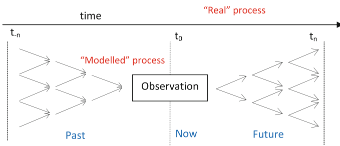
Fig. 1 “Modelled” process and “Real” process through time
