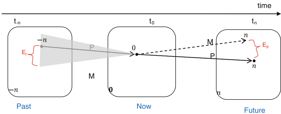
Fig. 4 Non-uniqueness and retrodiction
