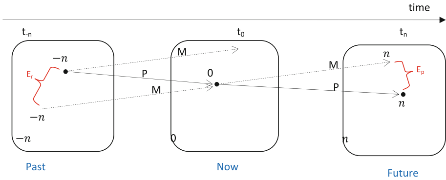
Fig. 3 Inverse process for M
