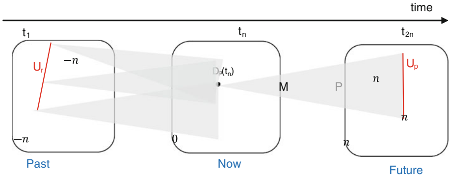
Fig. 5 The non-deterministic case
