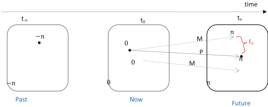
Fig. 2 Runs of M starting with different initial conditions
